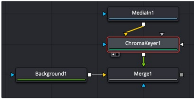
A Chroma Keyer node creating transparency on the MediaIn node
