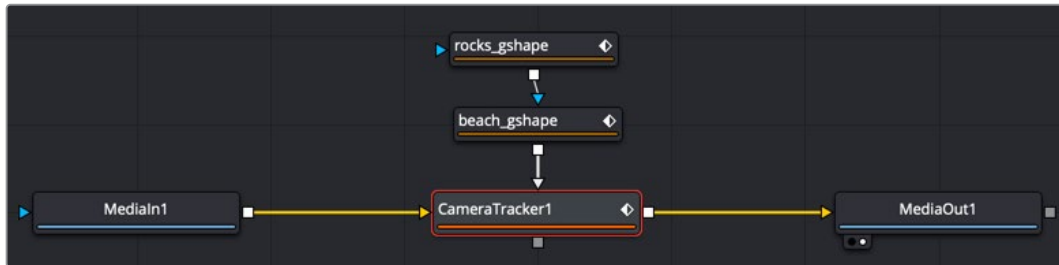
The Camera Tracker with occlusion masks
