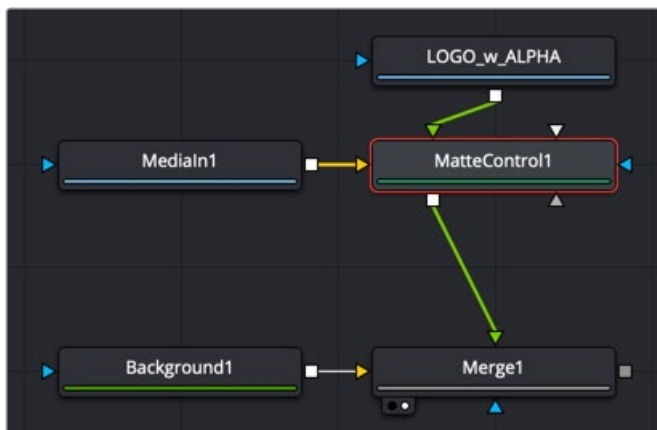
A Matte Control embedded an Alpha from the foreground input to the background input
