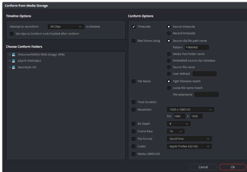
The Reconform From Media Storage dialog
