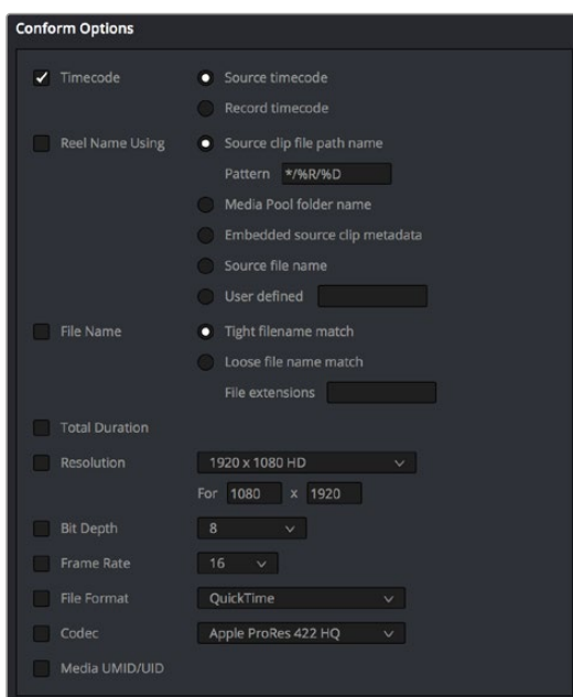
Selecting criteria to guide the reconform
